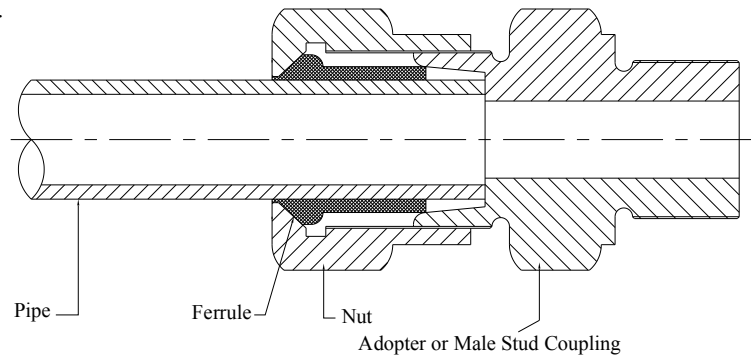
Figure No. 6.6 Ferrule Type Cmpression
