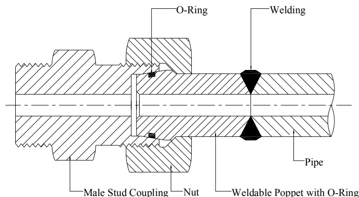
Figure No. 6.9 Threaded Type Welded End Fittings
