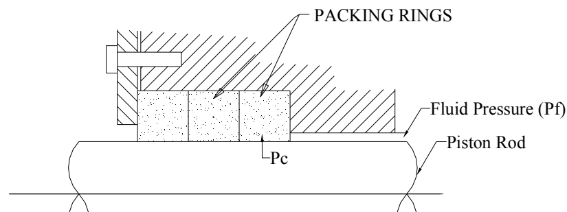
Figure No.7.1 Compression Sealing
