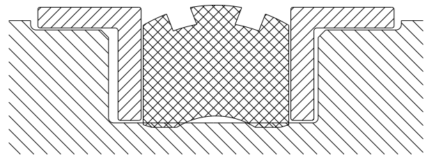
Trade Name - K17 - Double Acting Piston Seal
