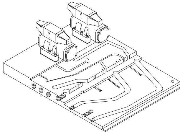
Figure 6.5 Gasket Moulded Manifold Block
