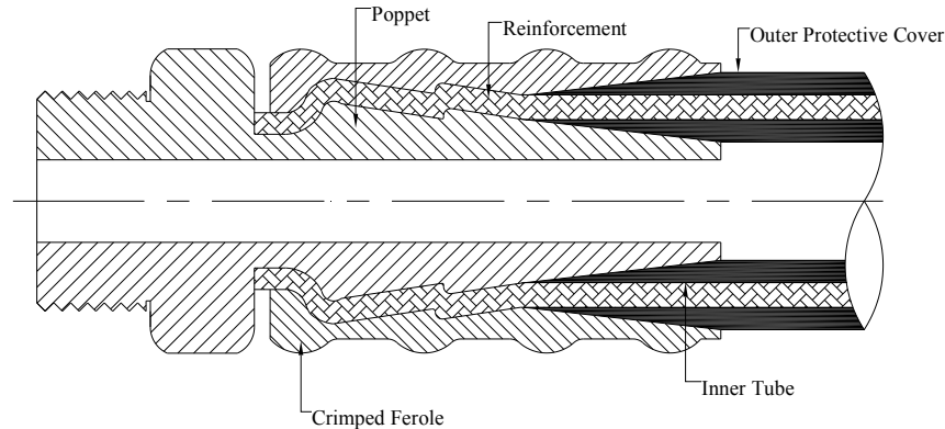
Figure No. 6.13 Permanently attached type End-Fitting
