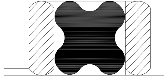
Quad Ring ® of Bushak+Shamban
