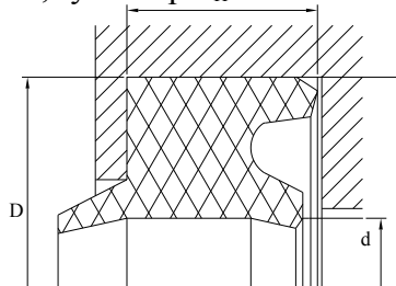
Trade Name - A11 Double lip Snap-in-Wiper
