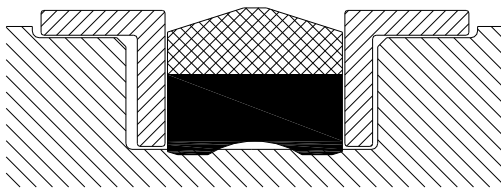
Trade Name - K9 - Double Acting Compact Piston Seal
