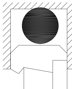
Trade name: S9 Composite rod seal Figure No.7.38 (b)
