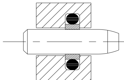
Rod seal installation sequence Figure No.7.21.1
