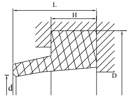
Trade Name - A2 Snap-in wiper hydraulic
