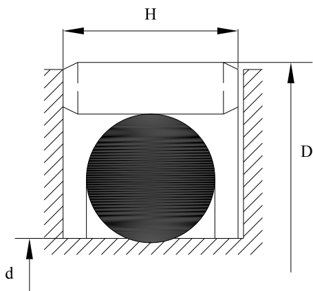
Trade name: K8 Composite piston seal Figure No.7.18.6 (a)
