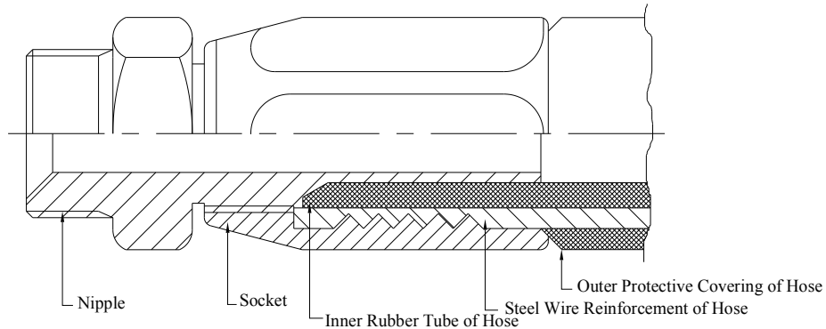
Figure No. 6.11 Re-usabile Type of End Fitting
