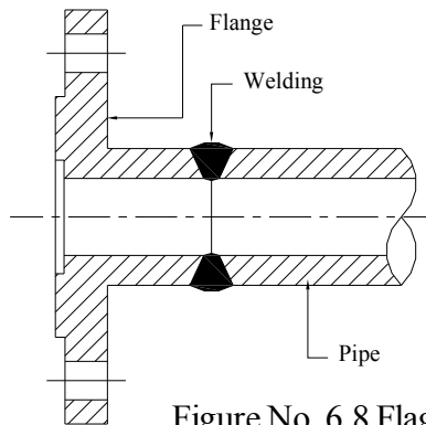
Figure No. 6.8 Flag Type Welded End Fittings
