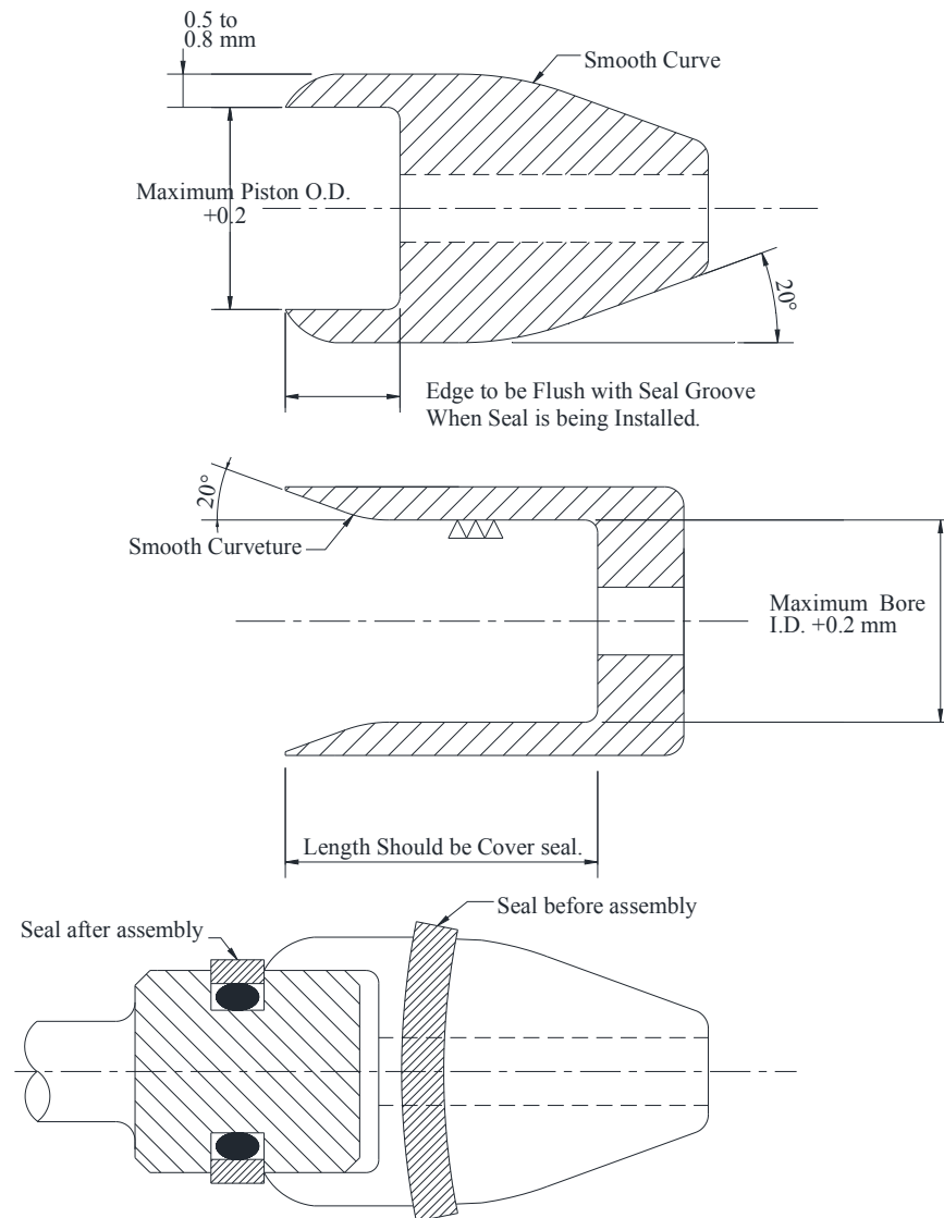
Figure No.7.54 Piston seal Installation Sequence
