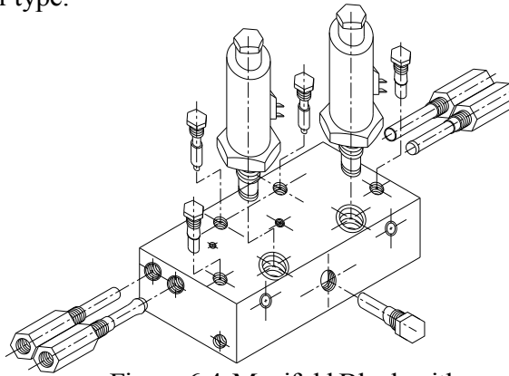
Figure 6.4 Manifold Block with Integrated Circuit fitted with Cartridge Valve
