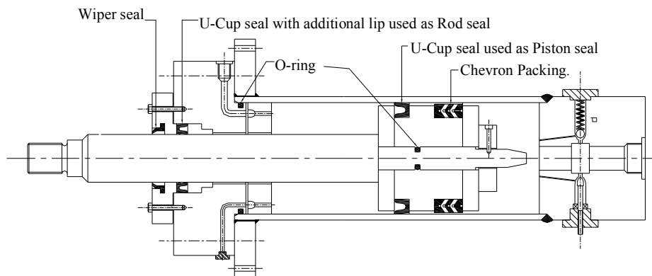
Figure No.7.12 Cross section of a Double Action Cylinder
