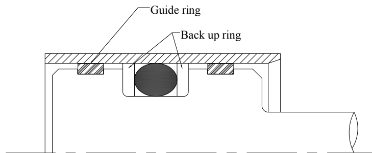
Figure No.7.25 Guide ring & Back-up ring
