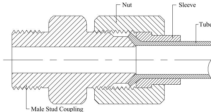
Figure No. 6.7 Threaded Flared Fitting
